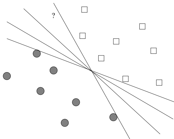
Figure 12.12: Generally, more than one hyperplane can separate the classes if they can be separated at all
